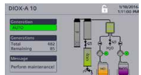
ANIMATED PROCESS FLOW SCHEME VIEW
