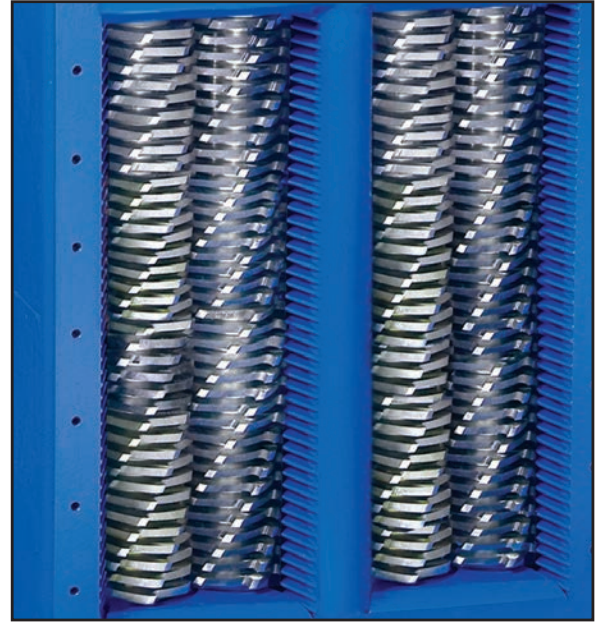
TM8532D Duplex is provided with twice the cutting capacity.
