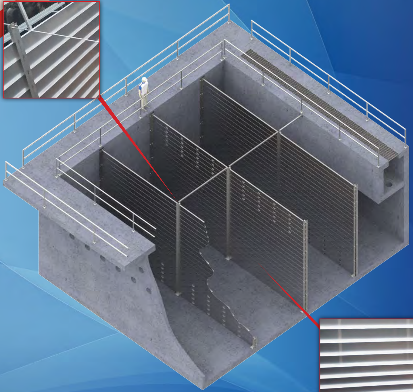
Connection Bar
